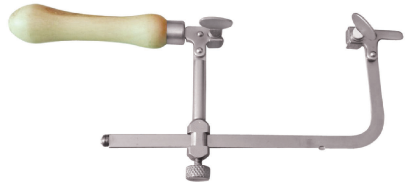
1000 Dental Laboratory Saw
